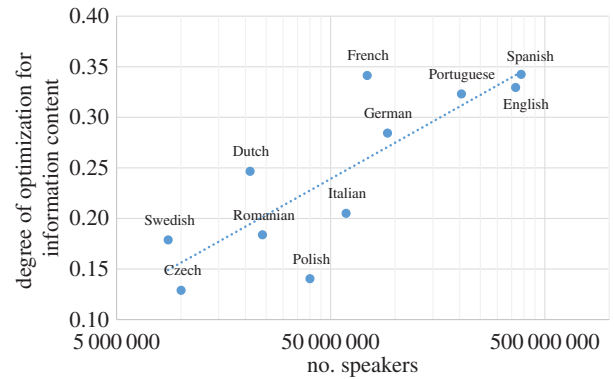
Figure 3. Relationship between the number of contemporary speakers of a language and the degree to which word lengths have been optimized for communication. The horizontal axis is a log scale. The vertical axis is the correlation between the information content of words and their written length made positive for easier interpretation. (Online version in colour.)
